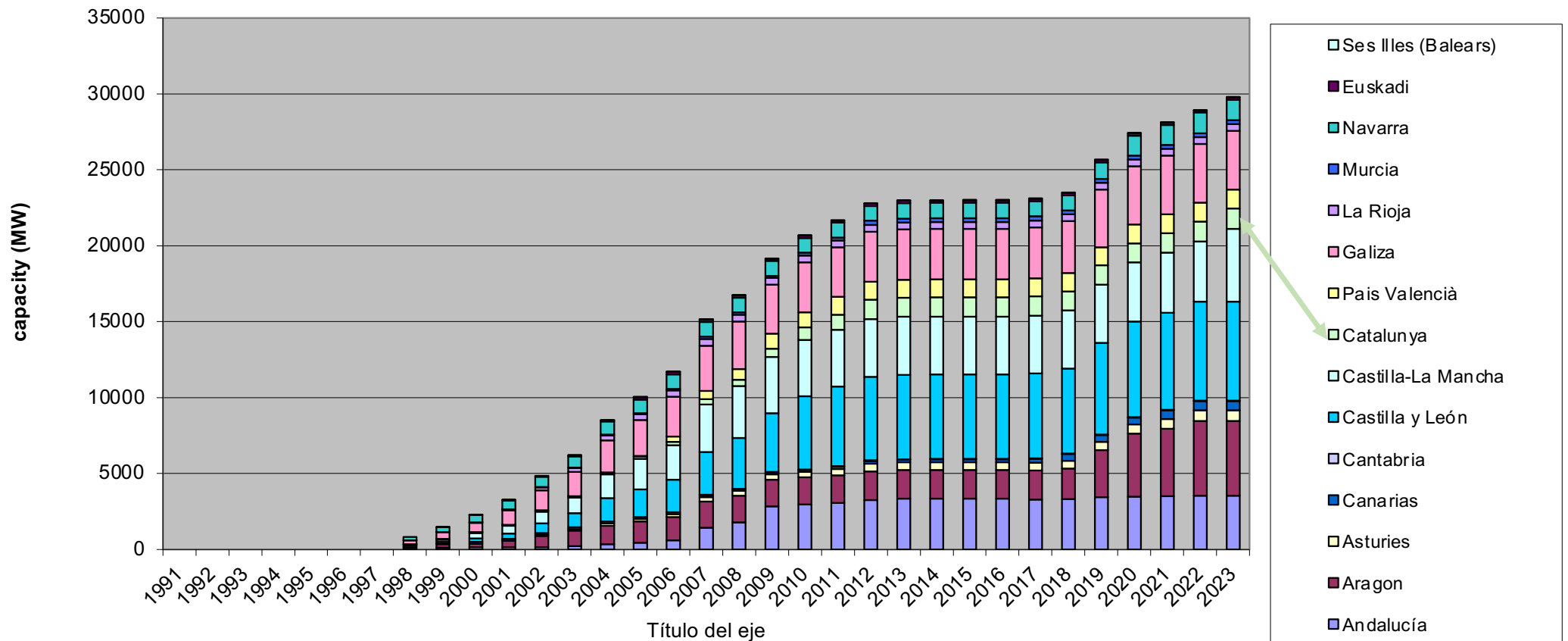
Wind Power Spain (1990-2023)
